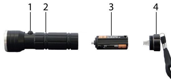
Fig. 10: Multi-function lamp (components)
