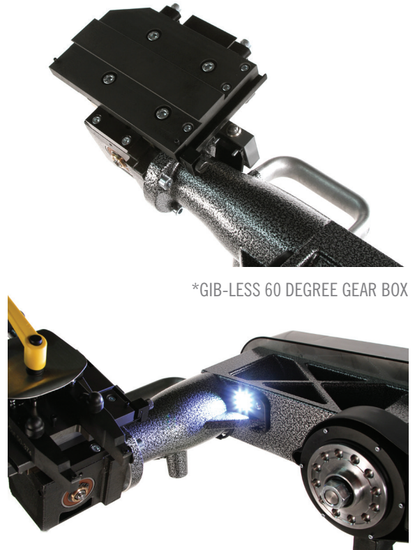
**6 LED ON-BOARD WORK LIGHT
