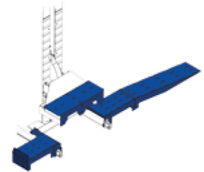
CLHM-FLA Fork Lift Adapter 15,000 lb. capacity used to raise fork lift 64"
